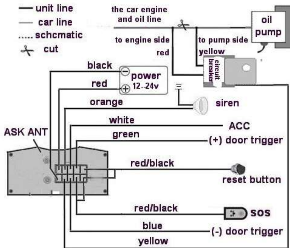
Wiring diagram
